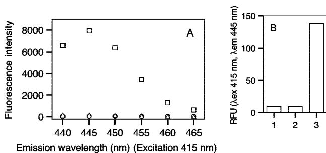
FIGURE 1. (A) Fluorescence emission spectra ( \lambda_{\text{ex}} 415 nm) of amine 1c (circle), imine 3c (triangle), and addition product 5c (square) at 5 \mu\text{M} in 5% DMSO/50 mM sodium phosphate, pH 7.0. (B) Fluorescence increase ( \lambda_{\text{ex}} 415 nm, \lambda_{\text{em}} 445 nm) after 70 min in 5% DMSO/50 mM sodium phosphate buffer, pH 7.0: column 1, phenol derivative 6 , 2.5 mM; column 2, imine 3c , 2.5 \mu\text{M} ; column 3, 6 , 2.5 mM and 3c , 2.5 \mu\text{M} .
